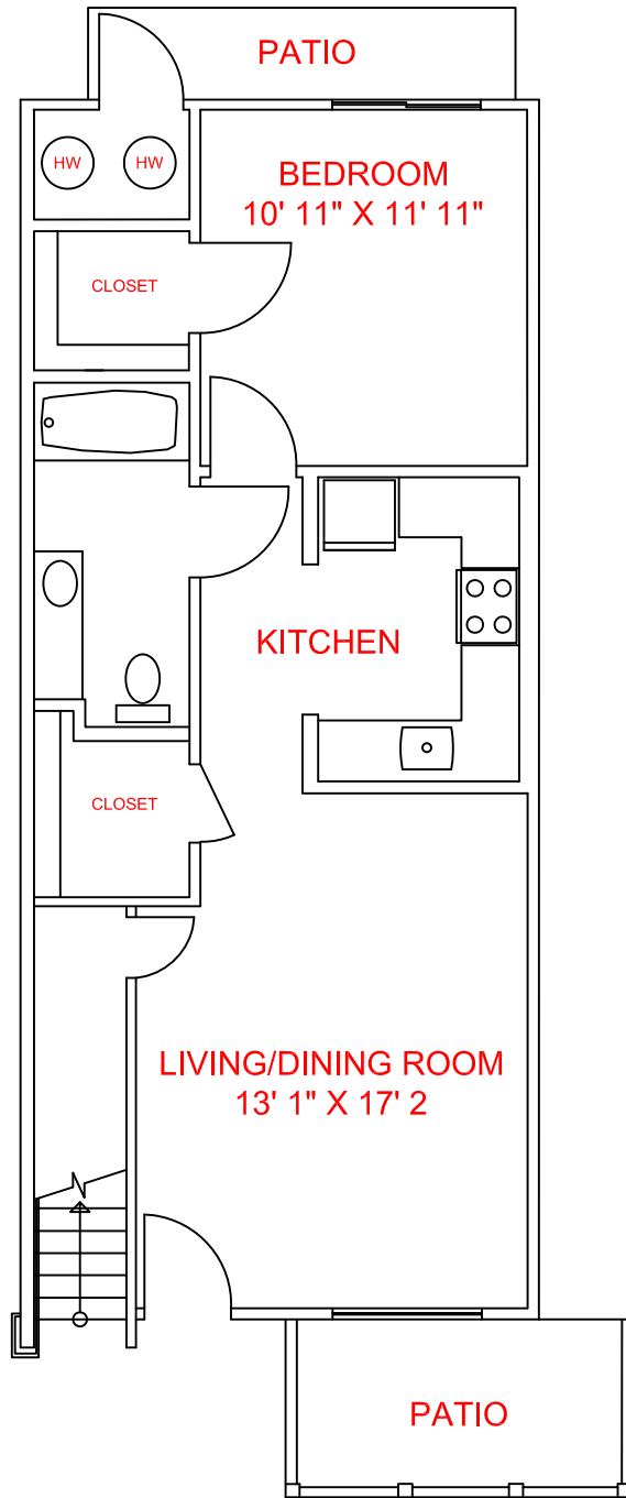
TYPE A - 1 BEDROOM 1st FLOOR
