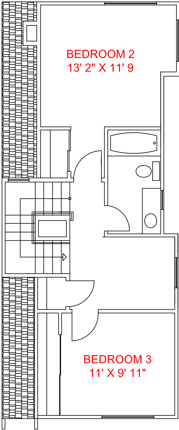
TYPE G 3 BEDROOM THIRD FLOOR
