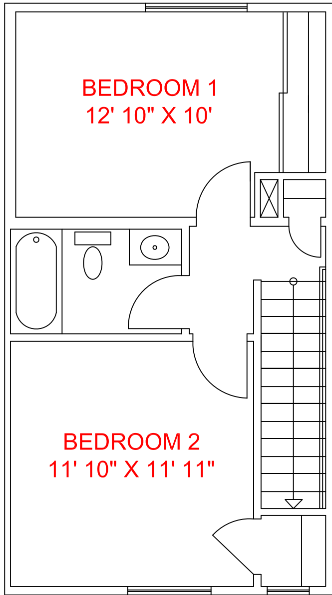
TYPE E - 2 BEDROOM SECOND FLOOR
