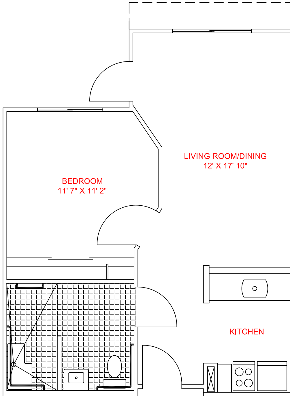
TYPE C - 1 BEDROOM DISABLED ACCESSIBLE
