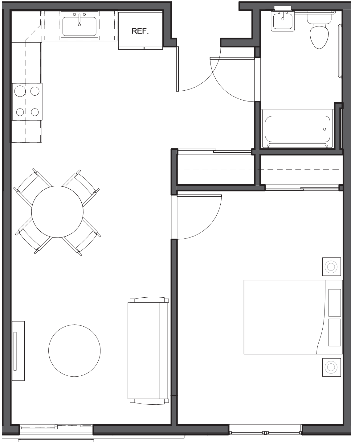
UNIT TYPE A1 608 SQ FT (84 UNITS)
