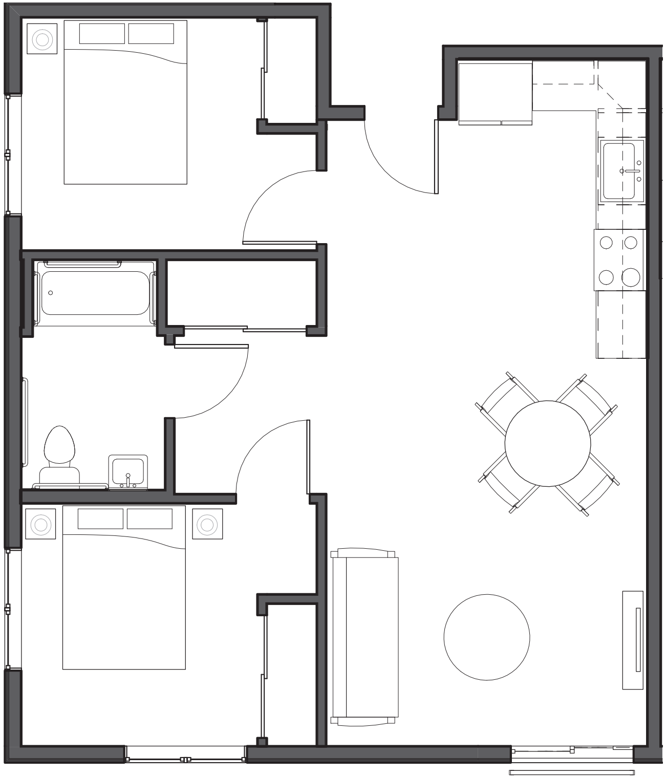
UNIT TYPE B1 718 SQ FT (3 UNITS)
