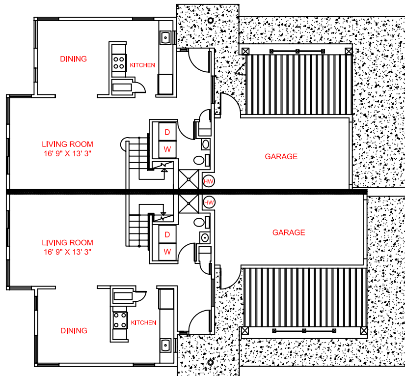
3 BEDROOM DUPLEX, GROUND FLOOR
