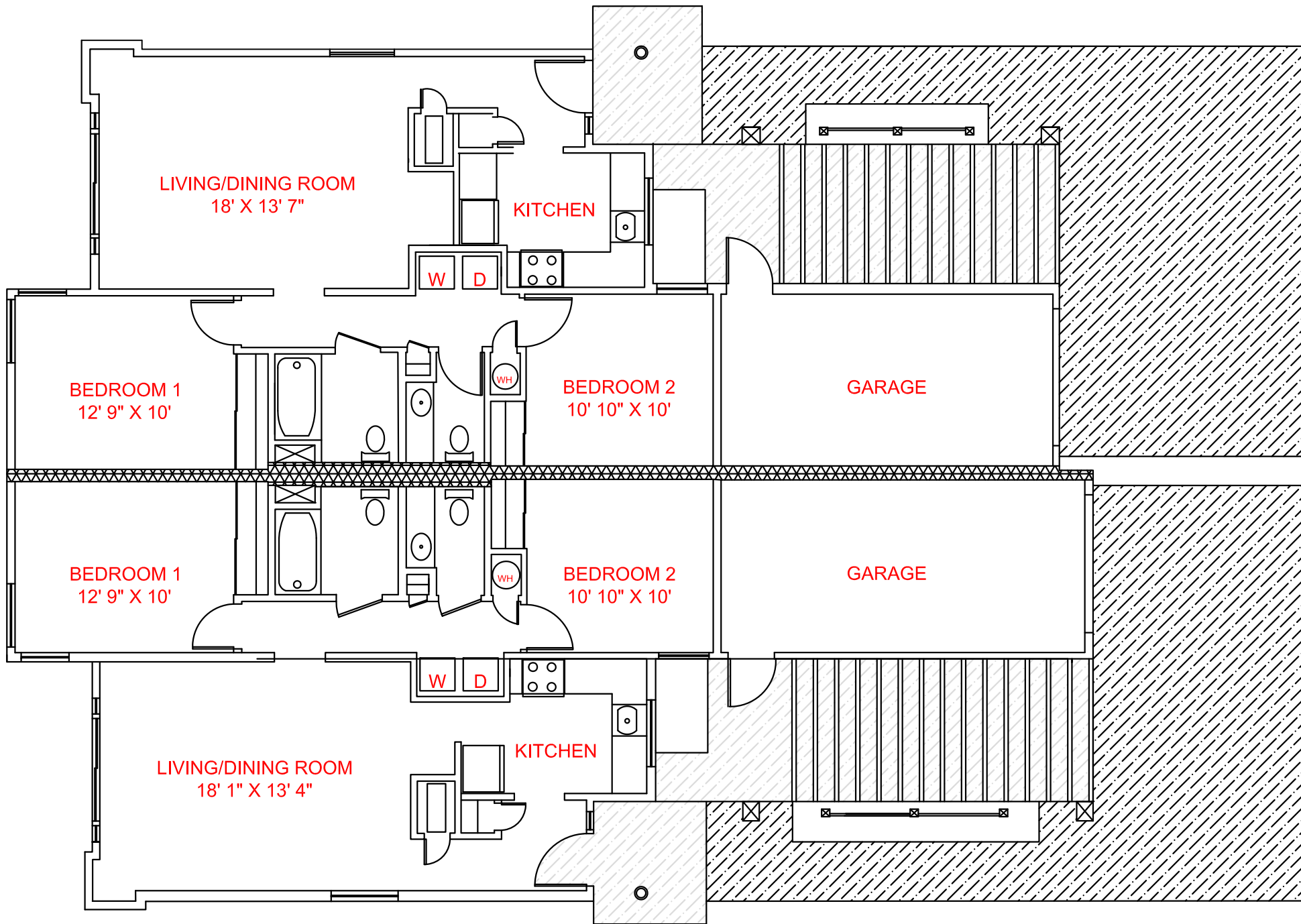
2 BEDROOM 1 1/2 BATH DUPLEX
