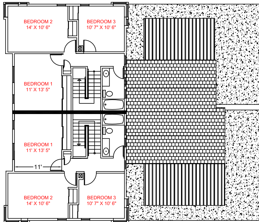
3 BEDROOM DUPLEX, UPPER FLOOR
