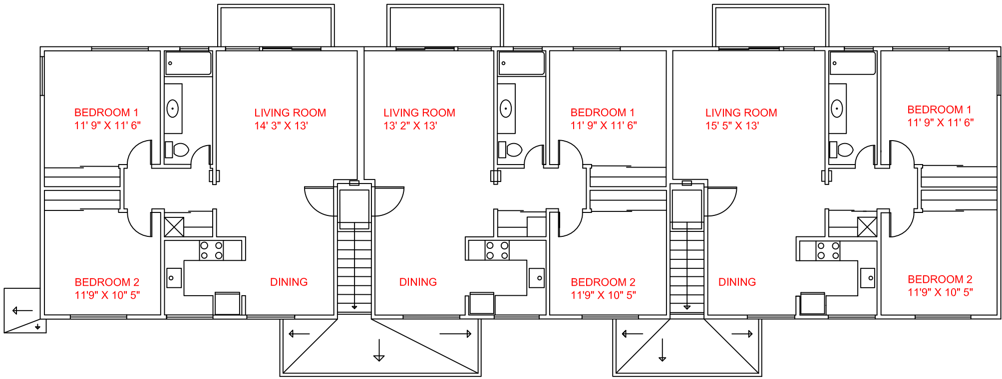
6 UNIT BUILDING SECOND FLOOR
