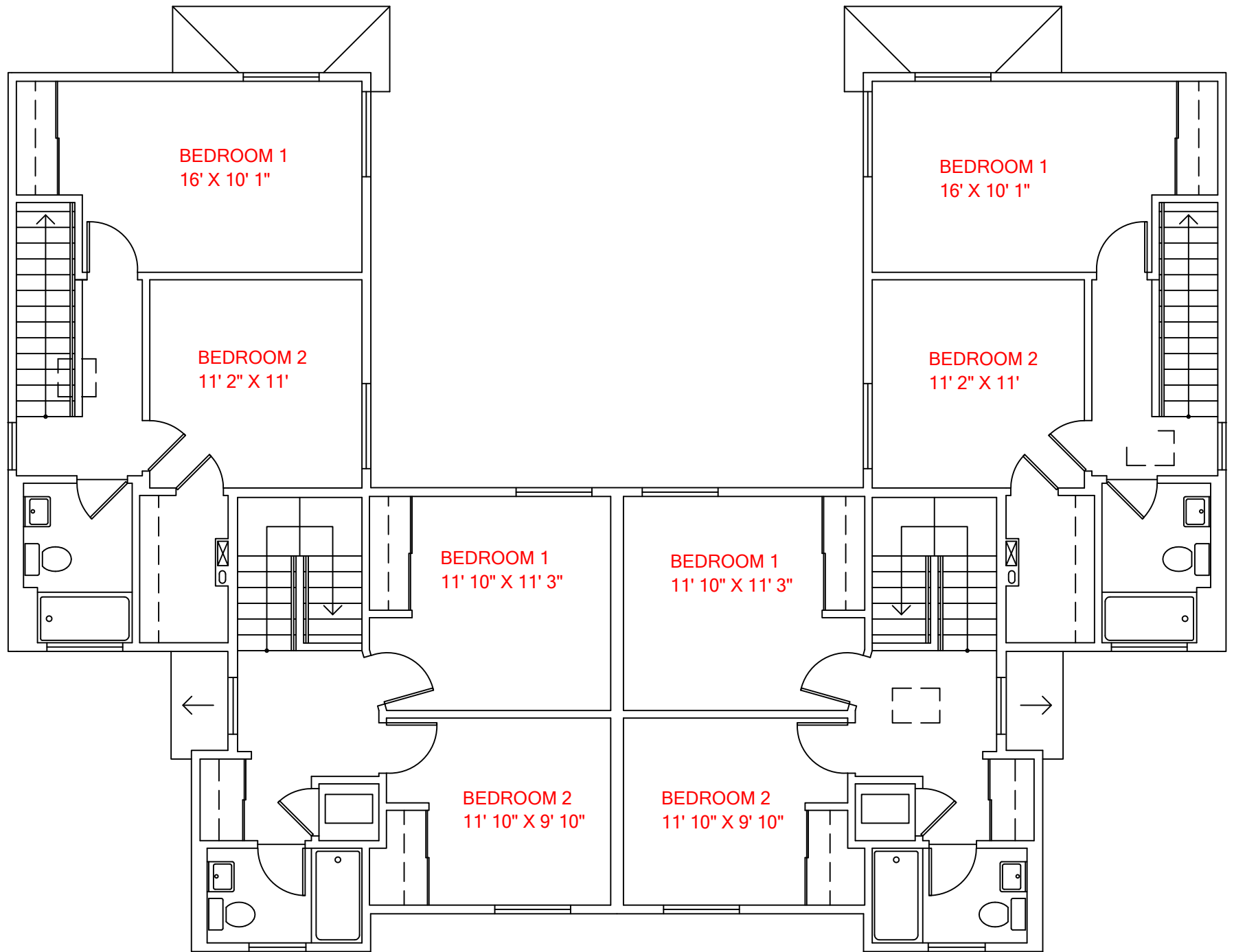
③ 3rd Floor, Building Type "C" Carport Building Type
