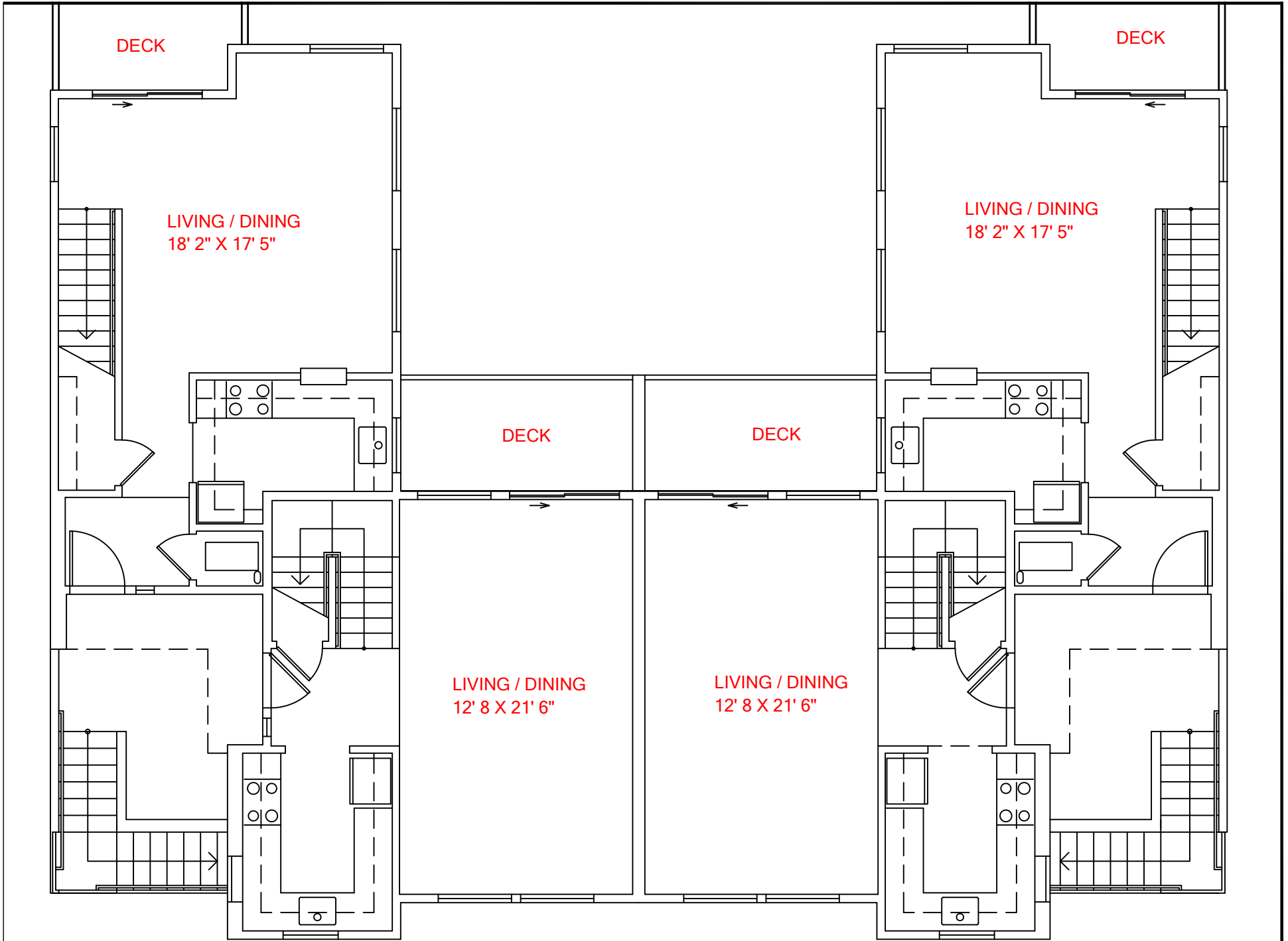
2nd Floor, Building Type "C" Carport Building Type
