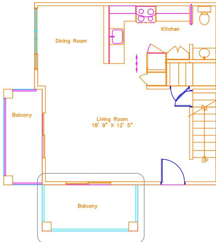
UNIT D LOWER LEVEL 2 B.R. 1 BATH
