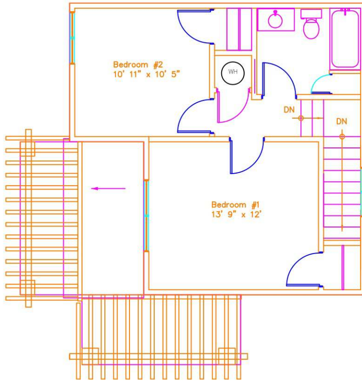
TYPICAL 2 B.R. TOWNHOUSE Upper Level
